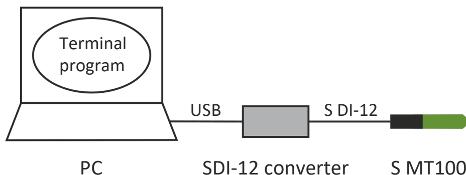
Figure 1: Hardware setup
